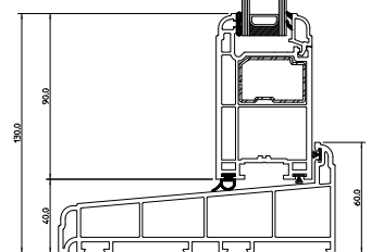
Sideways View - Deep Bottom Rail
