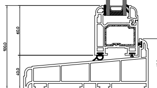
Sideways View - Standard Bottom Rail
